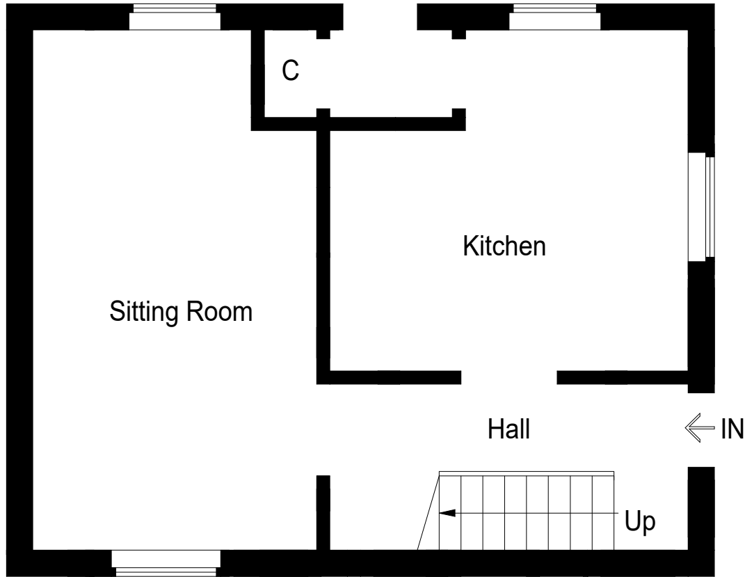
Ground Floor
